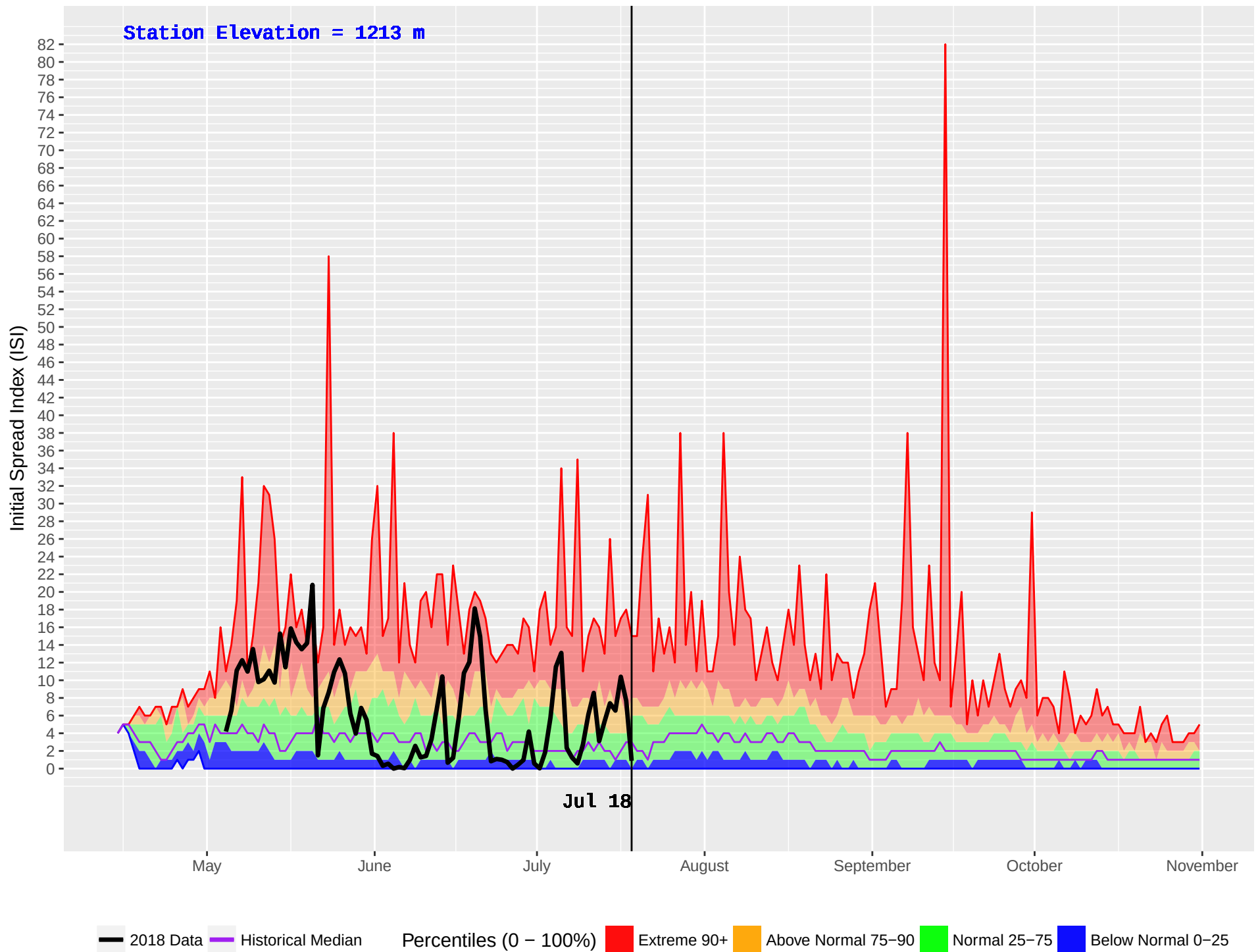
INGENIKA POINT (145) : Historical (1971–2016) and Current (2018) Daily Initial Spread Index (ISI)
