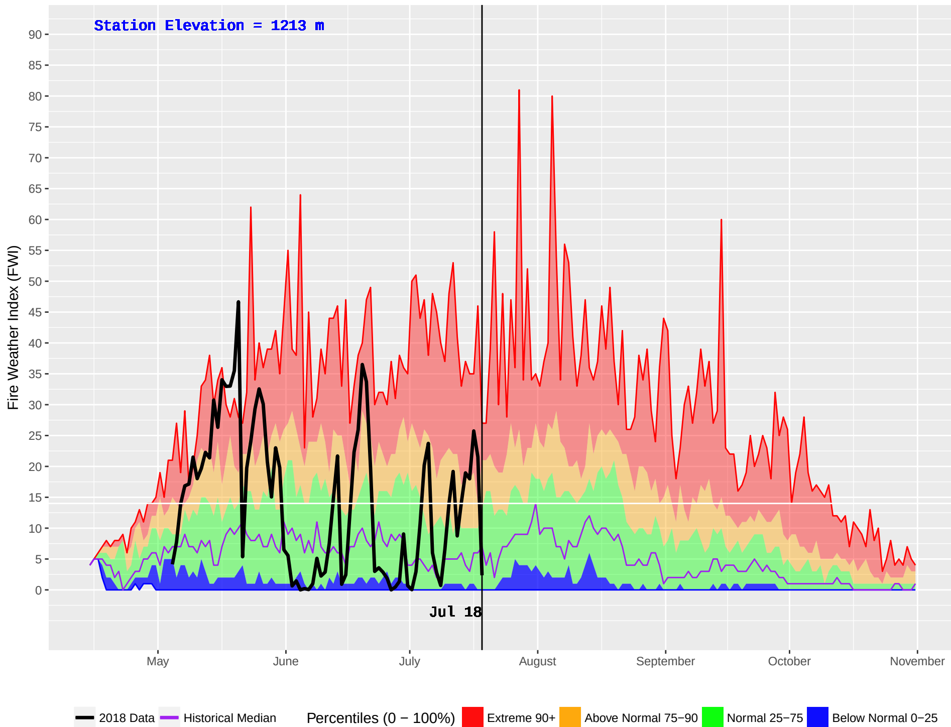
INGENIKA POINT (145) : Historical (1971–2016) and Current (2018) Daily Fire Weather Index (FWI)
