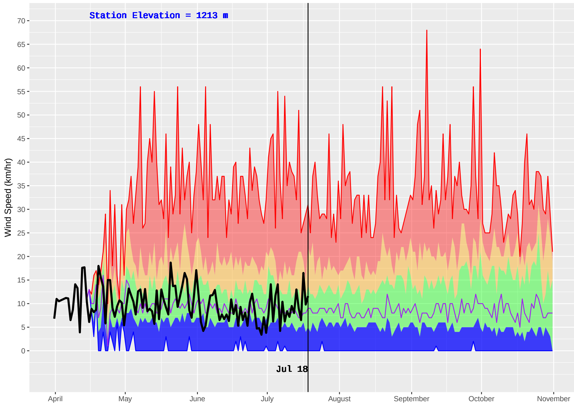
INGENIKA POINT (145) : Historical (1971–2016) and Current (2018) Daily Wind Speed
